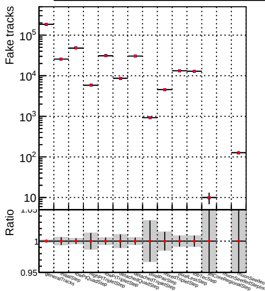
Number —●— DQM_V0001 R000000001 Global mkFit batch16
