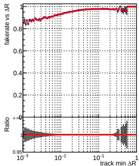
—•— DQM_V0001_R000000001_Global_mkFit_batchNO —•— DQM_V0001_R000000001_Global_mkFit_batch16
