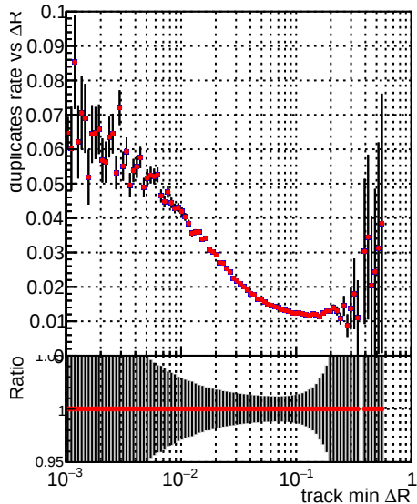
—•— DQM_V0001_R000000001_Global_mkFit_batchNO —•— DQM_V0001_R000000001_Global_mkFit_batch16
