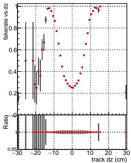
—●— DQM_V0001_R000000001_Global_mkFit_batchNO —●— DQM_V0001_R000000001_Global_mkFit_batch16
