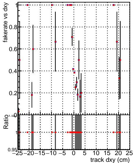
—●— DQM_V0001_R000000001_Global_mkFit_batchNO —●— DQM_V0001_R000000001_Global_mkFit_batch16
