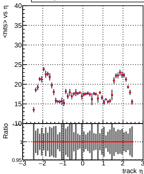
— DQM_V0001_R000000001_Global_mkFit_batchNO — DQM_V0001_R000000001_Global_mkFit_batch16
