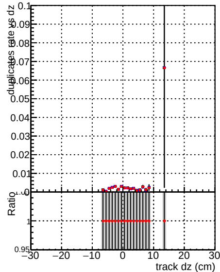
—●— DQM_V0001_R0000000001_Global_mkFit_batchNO —●— DQM_V0001_R0000000001_Global_mkFit_batch16
