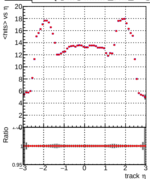
— DQM_V0001_R000000001_Global_mkFit_batchNO — DQM_V0001_R000000001_Global_mkFit_batch16
