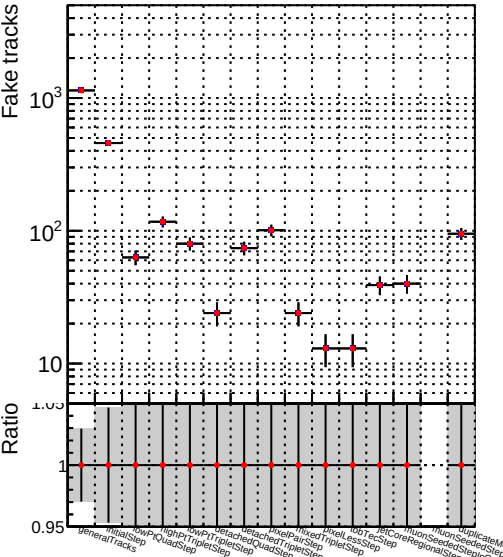
Number —●— DQM_V0001_R000000001_Global_mkFit_batch16
