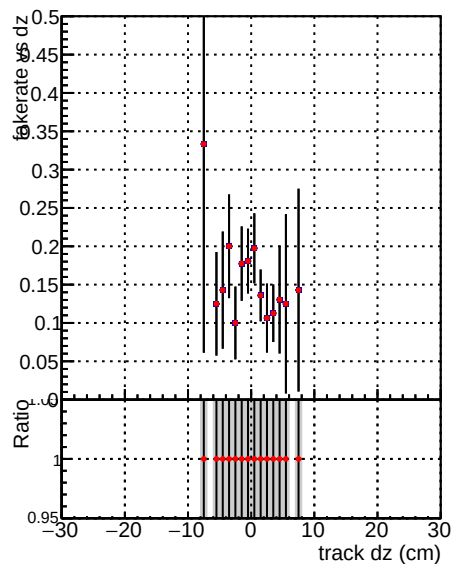
—●— DQM V0001_R000000001 Global mkFit batchNO —●— DQM V0001_R000000001 Global mkFit batch16
