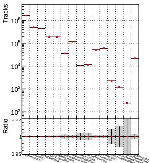
DQM_V0001_R000000001_Global_mkFit_batchNO
