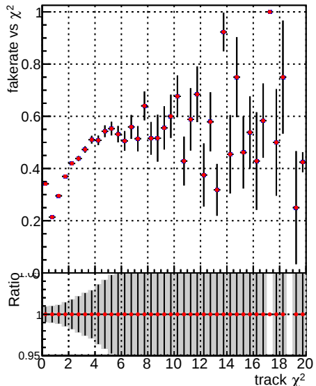
Fake rate vs. —•— DQM V0001_R000000001 Global mkFit batchNO —•— DQM V0001_R000000001 Global mkFit batch16
