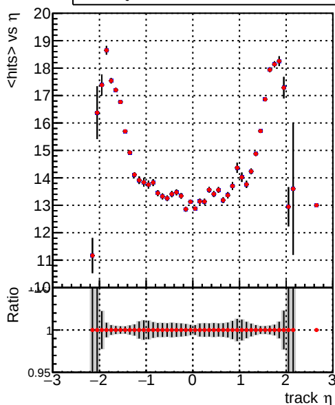
mean hits vs \eta — DQM_V0001_R000000001_Global_mkFit_batchNO — DQM_V0001_R000000001_Global_mkFit_batch16
