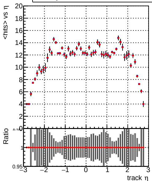
— DQM_V0001_R000000001_Global_mkFit_batchNO — DQM_V0001_R000000001_Global_mkFit_batch16
