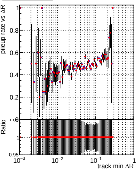
Legend: DQM_V0001_R000000001_Global_mkFit_batchNO (blue), DQM_V0001_R000000001_Global_mkFit_batch16 (red)
