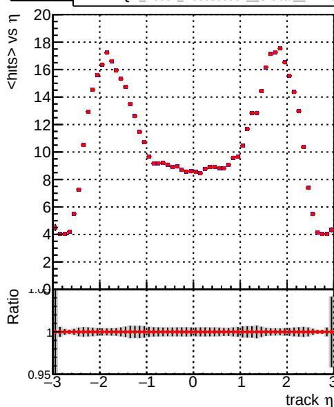
— DQM_V0001_R000000001_Global_mkFit_batchNO — DQM_V0001_R000000001_Global_mkFit_batch16
