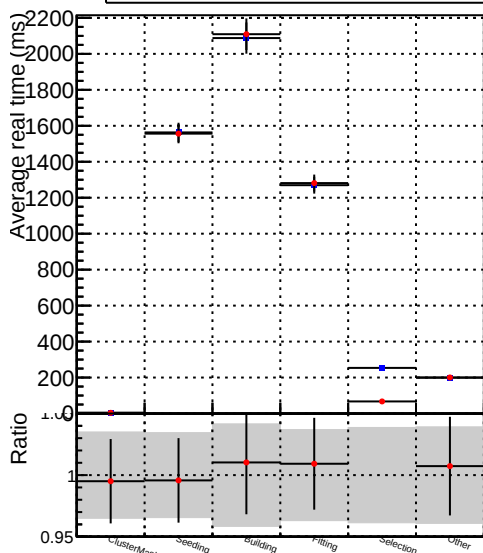
Average —●— DQM_V0001_R000000001_Global_mkFit_batch16-100
