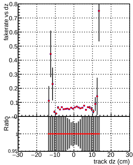
Fake rate vs dz DQM V0001_R000000001 Global mkFit batchNO-100 DQM V0001_R000000001 Global mkFit batch16-100
