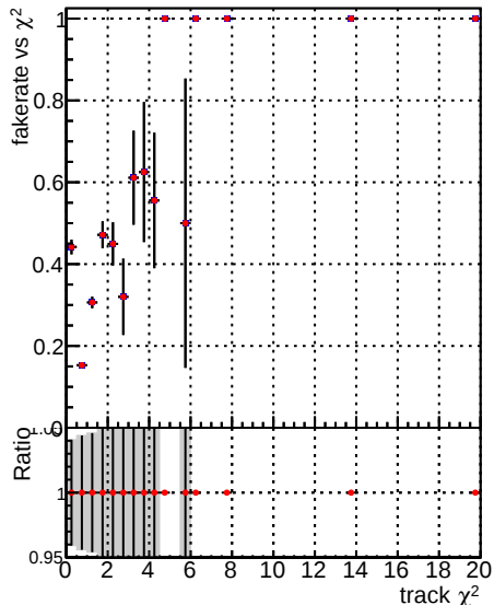
Fake rate vs. —•— DQM_V0001_R0000000001_Global_mkFit_batchNO-100 —•— DQM_V0001_R0000000001_Global_mkFit_batch16-100
