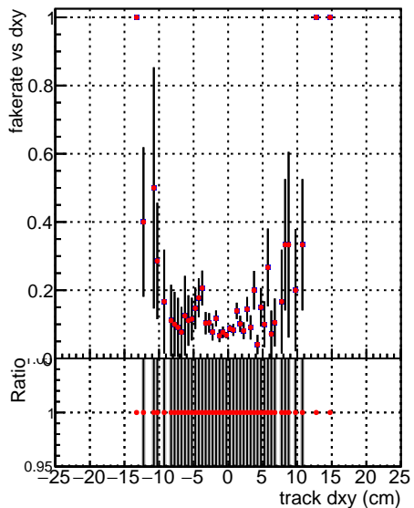
—●— DQM_V0001_R000000001_Global_mkFit_batchNO-100 —●— DQM_V0001_R000000001_Global_mkFit_batch16-100
