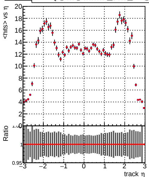
— DQM_V0001_R000000001_Global_mkFit_batchNO-100 — DQM_V0001_R000000001_Global_mkFit_batch16-100
