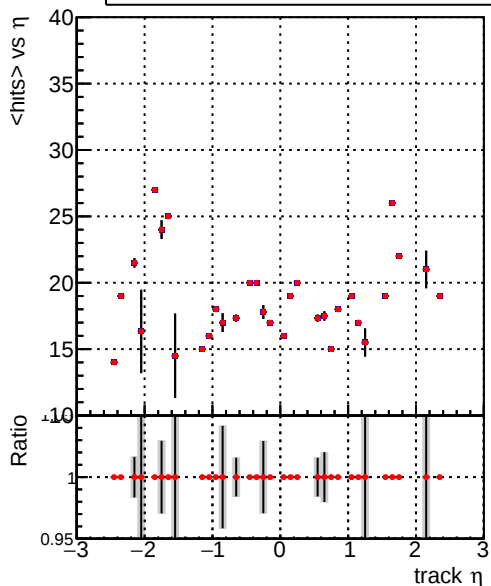
mean hits vs \eta — DQM_V0001_R000000001_Global_mkFit_batchNO-100 — DQM_V0001_R000000001_Global_mkFit_batch16-100
