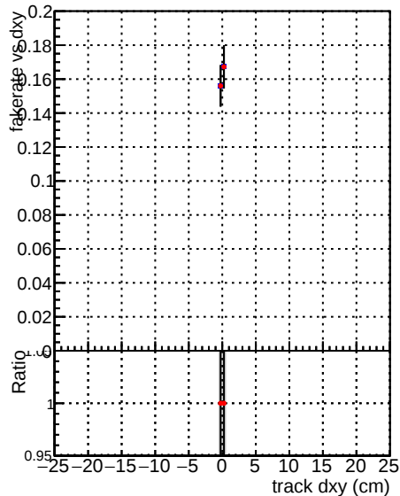
—•— DQM_V0001_R0000000001_Global_mkFit_batchNO-100 —•— DQM_V0001_R0000000001_Global_mkFit_batch16-100
