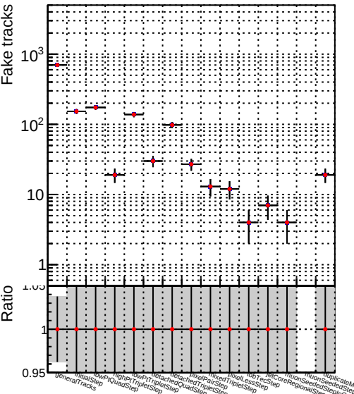
Number —●— DQM_V0001_R000000001_Global_mkFit_batch16-100
