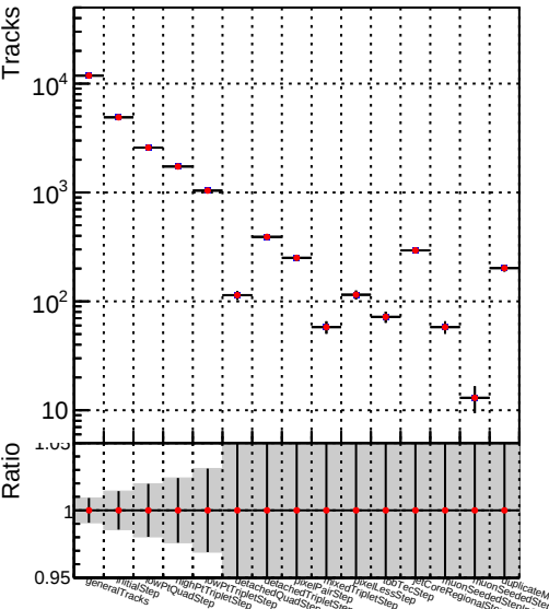
■ DQM_V0001_R000000001_Global_mkFit_batchNO-100
