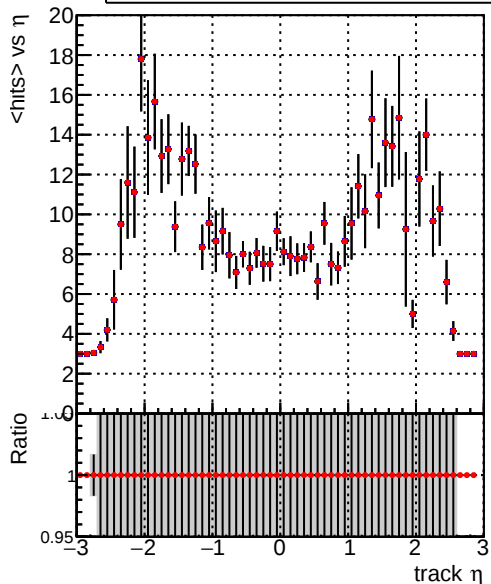
— DQM_V0001_R0000000001_Global_mkFit_batchNO-100 — DQM_V0001_R0000000001_Global_mkFit_batch16-100
