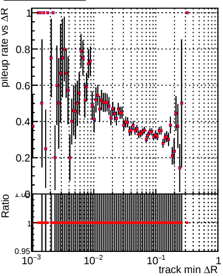
—•— DQM_V0001_R000000001_Global_mkFit_batchNO-100 —•— DQM_V0001_R000000001_Global_mkFit_batch16-100
