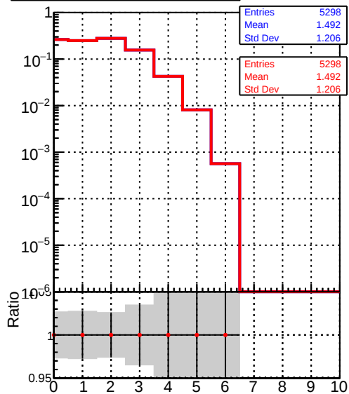
— DQM_V0001_R000000001_Global_mkFit_batchNO-100 — DQM_V0001_R000000001_Global_mkFit_batch16-100
