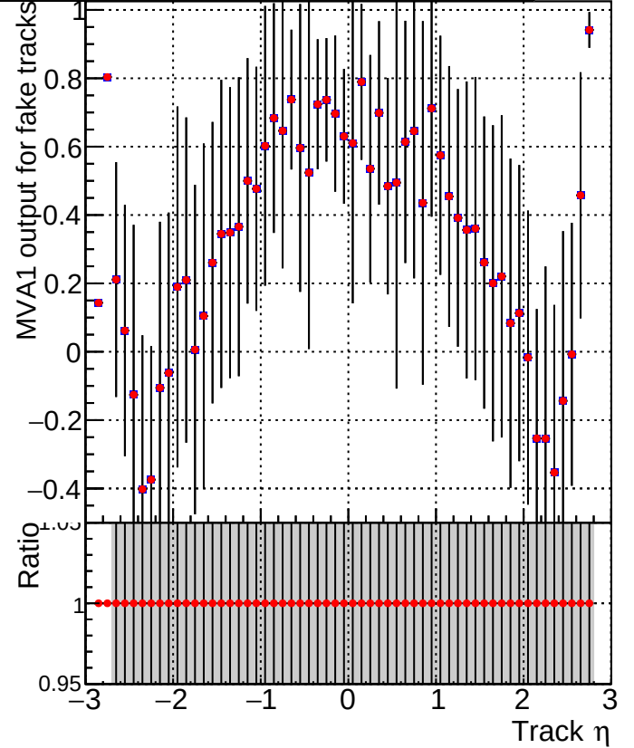
MVA1 of associated tracks (recoToSim) vs. track \eta ■ DQM_V0001_R000000001_Global_mkFit_batchNO-100 ● DQM_V0001_R000000001_Global_mkFit_batch16-100
