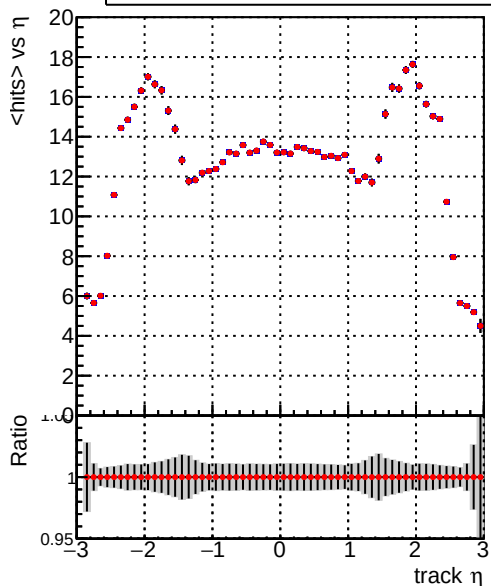
mean hit — DQM_V0001_R000000001_Global_mkFit_batchNO-100 — DQM_V0001_R000000001_Global_mkFit_batch16-100
