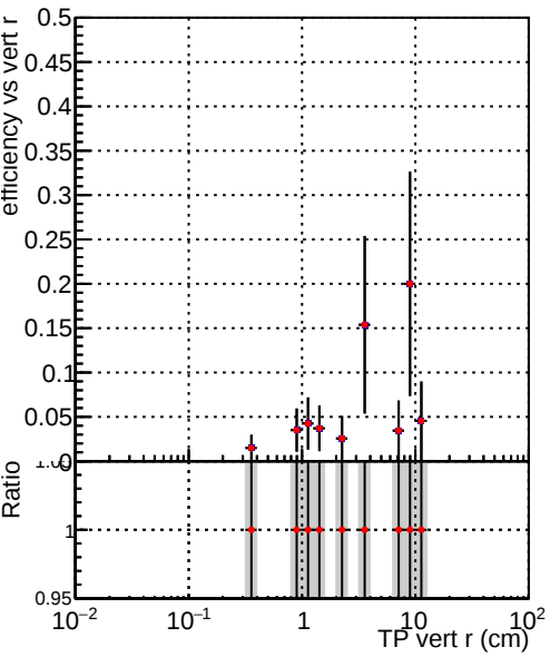
Efficiency vs. TP vert r (cm) Legend: DQM_V0001_R000000001_Global_mkFit_batchNO-100 DQM_V0001_R000000001_Global_mkFit_batch16-100
