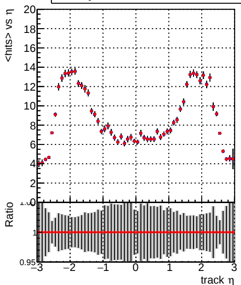
— DQM_V0001_R000000001_Global_mkFit_batchNO-100 — DQM_V0001_R000000001_Global_mkFit_batch16-100
