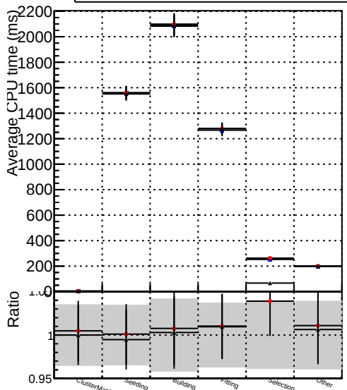
Average CPU time / event
