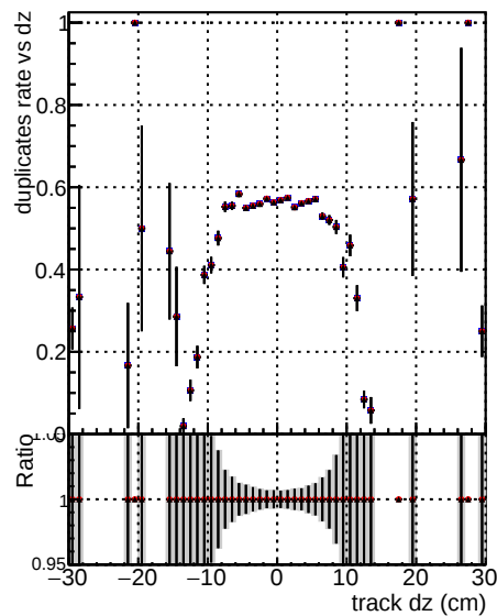
Legend: DOM V0001 R0000000001 Global mkFit batchNO_100 DOM V0001 R0000000001 Global mkFit batchNO_100-function DOM V0001 R0000000001 Global mkFit batch16-100-function
