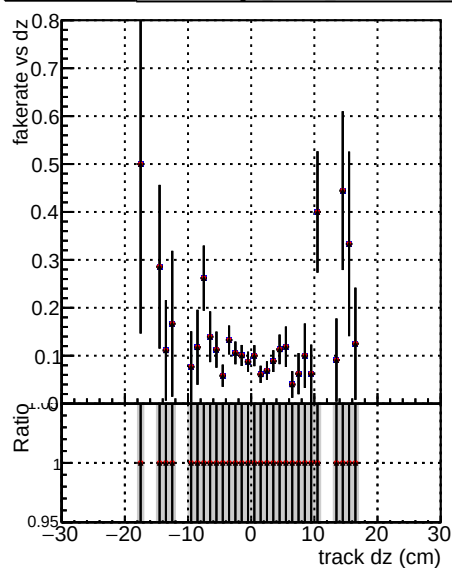
Legend for Fake rate vs dz, Duplicates rate vs dz, and Pileup rate vs dz plots: DOM V0001 R0000000001 Global mkFit batchNO_100 DOM V0001 R0000000001 Global mkFit batchNO_100-function DOM V0001 R0000000001 Global mkFit batch16-100-function
