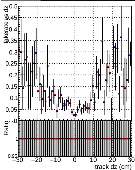
Legend for Fake rate vs d, Duplicates rate vs dz, and Pileup rate vs dz plots: DOM V0001 R0000000001 Global mkFit batchNO-100 DOM V0001 R0000000001 Global mkFit batchNO-100-function DOM V0001 R0000000001 Global mkFit batch16-100-function
