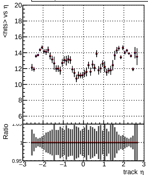
mean hits vs \eta DQM_V0001_R000000001_Global_mkFit_batchNO-100 DQM_V0001_R000000001_Global_mkFit_batchNO-100-function DQM_V0001_R000000001_Global_mkFit_batch16-100-function
