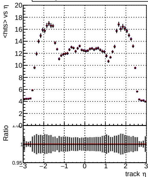
mean hits vs \eta DQM_V0001_R000000001_Global_mkFit_batchNO-100 DQM_V0001_R000000001_Global_mkFit_batchNO-100-function DQM_V0001_R000000001_Global_mkFit_batch16-100-function
