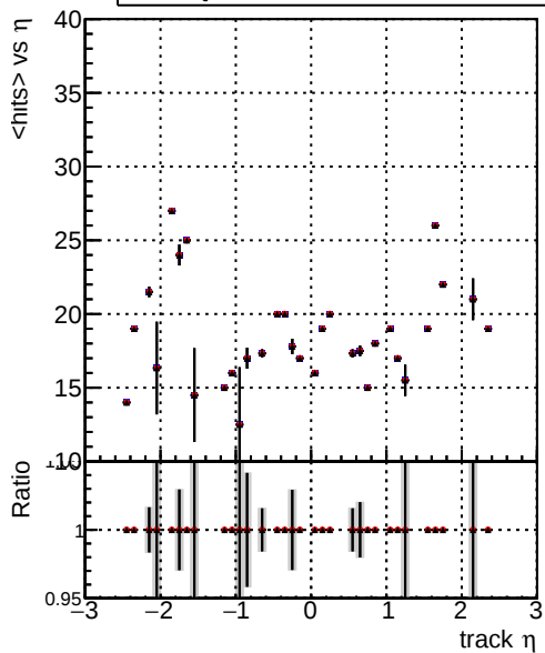
mean hits > \eta — DQM_V0001_R000000001_Global_mkFit_batchNO-100 — DQM_V0001_R000000001_Global_mkFit_batchNO-100-function — DQM_V0001_R000000001_Global_mkFit_batch16-100-function
