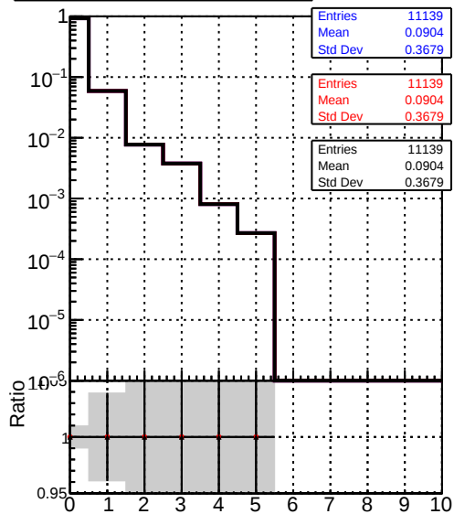
mean hit DQM_V0001_R000000001_Global_mkFit_batchNO-100 DQM_V0001_R000000001_Global_mkFit_batchNO-100-function DQM_V0001_R000000001_Global_mkFit_batch16-100-function
