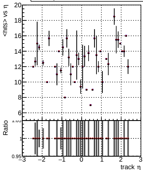
mean hit DQM_V0001_R0000000001_Global_mkFit_batchNO-100 DQM_V0001_R0000000001_Global_mkFit_batchNO-100-function DQM_V0001_R0000000001_Global_mkFit_batch16-100-function
