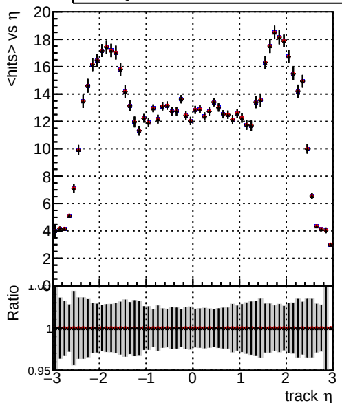
mean hit DQM_V0001_R000000001_Global_mkFit_batchNO-100 DQM_V0001_R000000001_Global_mkFit_batchNO-100-function DQM_V0001_R000000001_Global_mkFit_batch16-100-function
