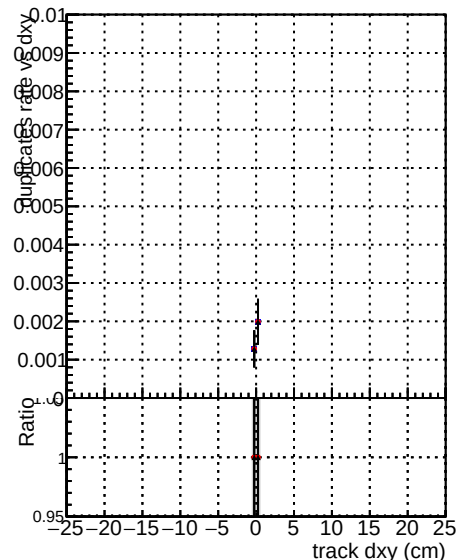
DOM V0001 R0000000001 Global mkFit batchNO_100 DOM V0001 R0000000001 Global mkFit batchNO_100-function DOM V0001 R0000000001 Global mkFit batch16-100-function
