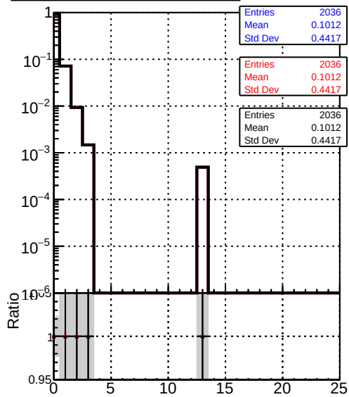
mean hits > \eta — DQM_V0001_R000000001_Global_mkFit_batchNO-100 — DQM_V0001_R000000001_Global_mkFit_batchNO-100-function — DQM_V0001_R000000001_Global_mkFit_batch16-100-function
