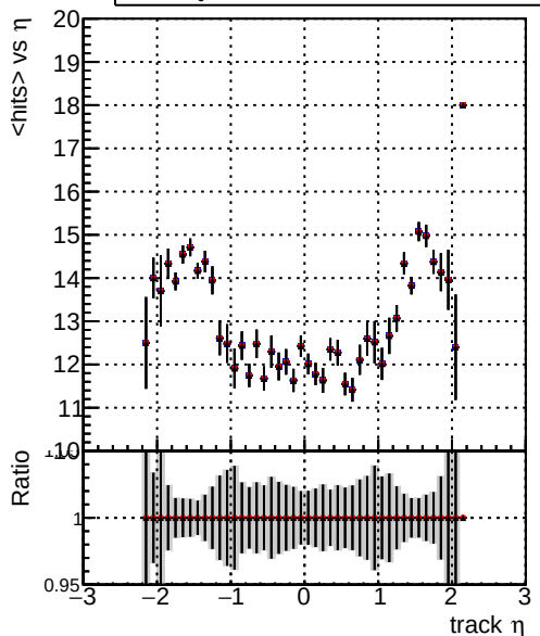
mean hits — DQM_V0001_R000000001_Global_mkFit_batchNO-100 — DQM_V0001_R000000001_Global_mkFit_batchNO-100-function — DQM_V0001_R000000001_Global_mkFit_batch16-100-function
