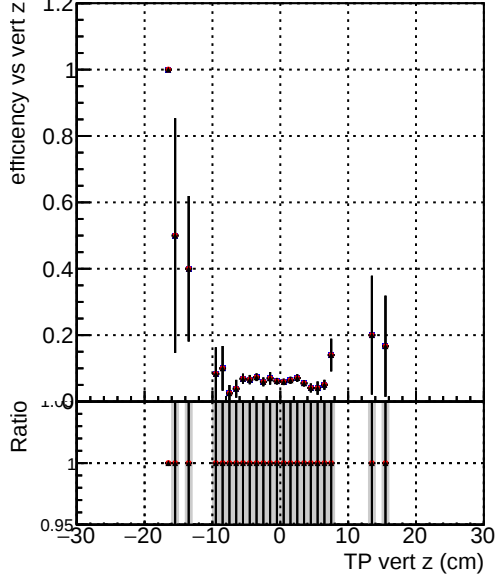
Efficiency vs vert z —●— DQM_V0001_R0000000001_Global_mkFit_batchNO-100 —●— DQM_V0001_R0000000001_Global_mkFit_batchNO-100-function —●— DQM_V0001_R0000000001_Global_mkFit_batch16-100-function
