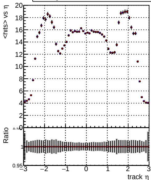
mean hits > \eta — DQM_V0001_R000000001_Global_mkFit_batchNO-100 — DQM_V0001_R000000001_Global_mkFit_batchNO-100-function — DQM_V0001_R000000001_Global_mkFit_batch16-100-function
