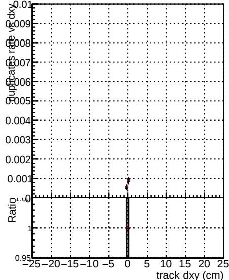
Legend for Fake rate vs d, Duplicates Rate vs Dxy, and Pileup rate vs dxy: DOM V0001 R0000000001 Global mkFit batchNO_100 DOM V0001 R0000000001 Global mkFit batchNO_100-function DOM V0001 R0000000001 Global mkFit batch16-100-function
