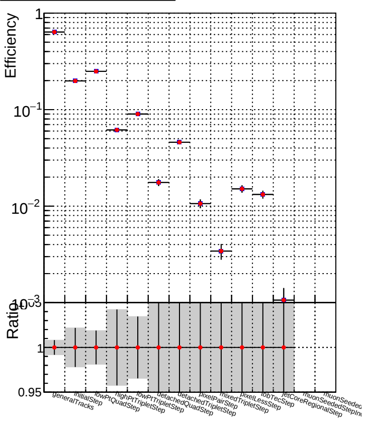
DQM_V0001_R000000001_Global_mkFit_nobatch DQM_V0001_R000000001_Global_mkFit_maybebatch
