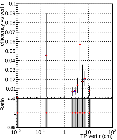
Efficiency vs vertpos Legend: DQM_V0001_R000000001_Global_mkFit_nobatch DQM_V0001_R000000001_Global_mkFit_maybepoch
