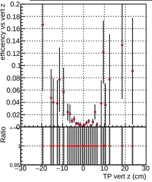
Efficiency vs vertpos Legend: DQM_V0001_R000000001_Global_mkFit_nobatch DQM_V0001_R000000001_Global_mkFit_maybebatch
