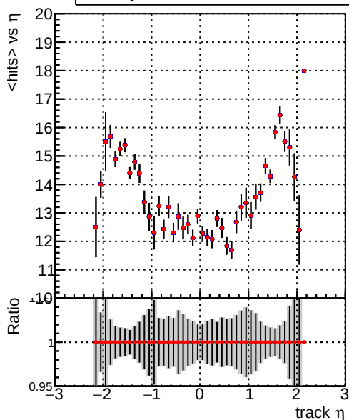
mean hit — DQM_V0001_R000000001_Global_mkFit_nobatch — DQM_V0001_R000000001_Global_mkFit_maybepoch
