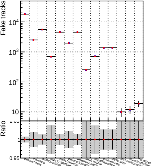
Number ● DQM_V0001_R0000000001_Global_mkFit_maybebatch
